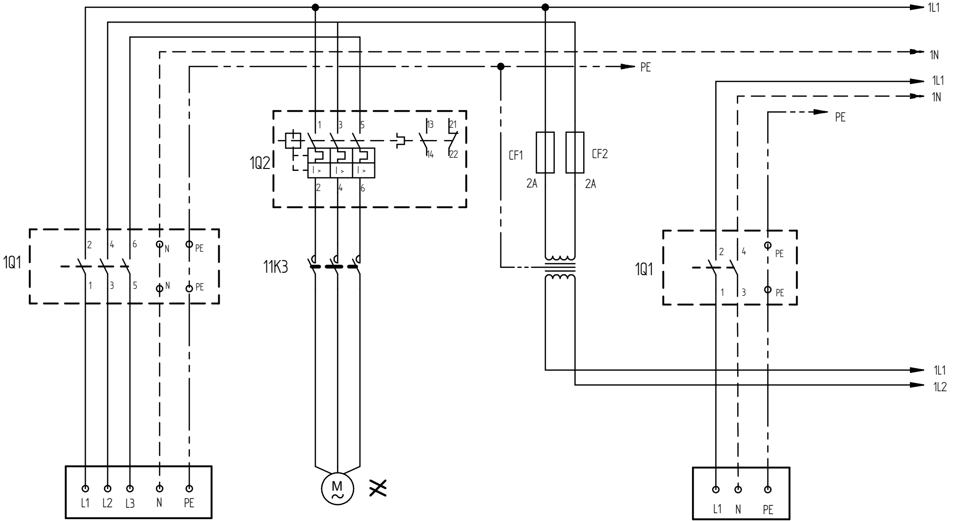
CONTROL TRANSFORMER
